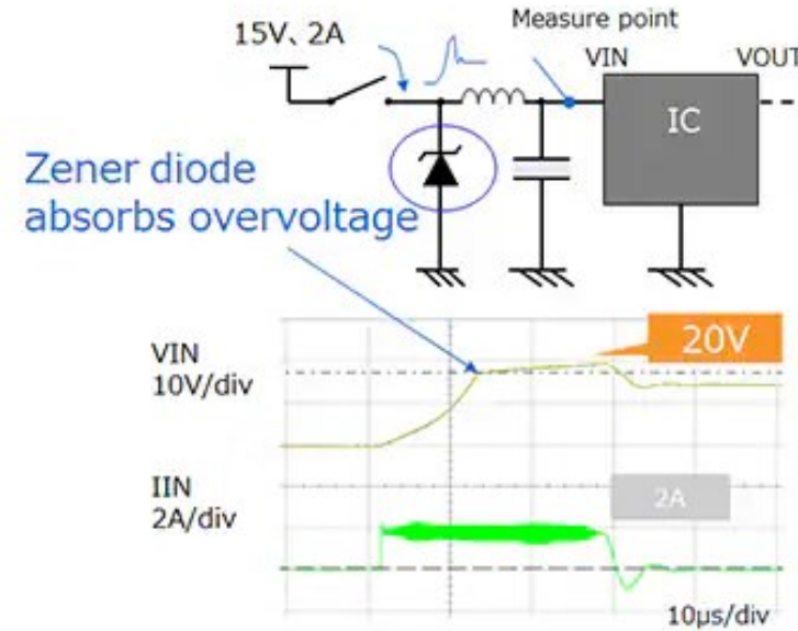
With Zener Diode
