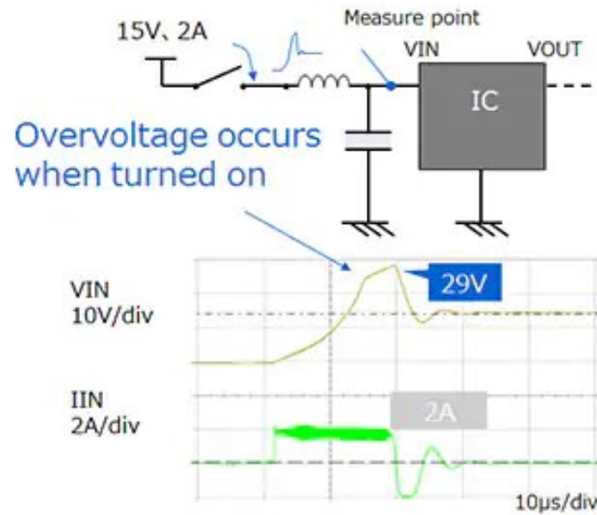
Without Zener Diode
