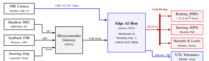
Fig. 1. In-cabin hardware wiring and system bus topology
