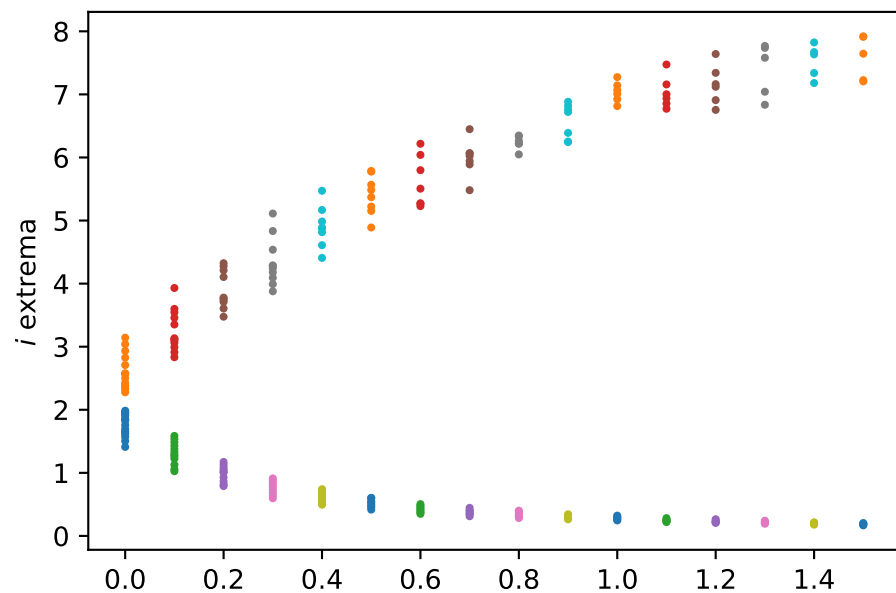
(c) hunting efficiency \beta
