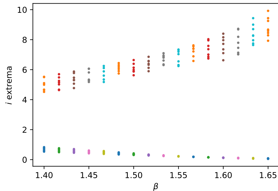
(c) hunting efficiency \beta
