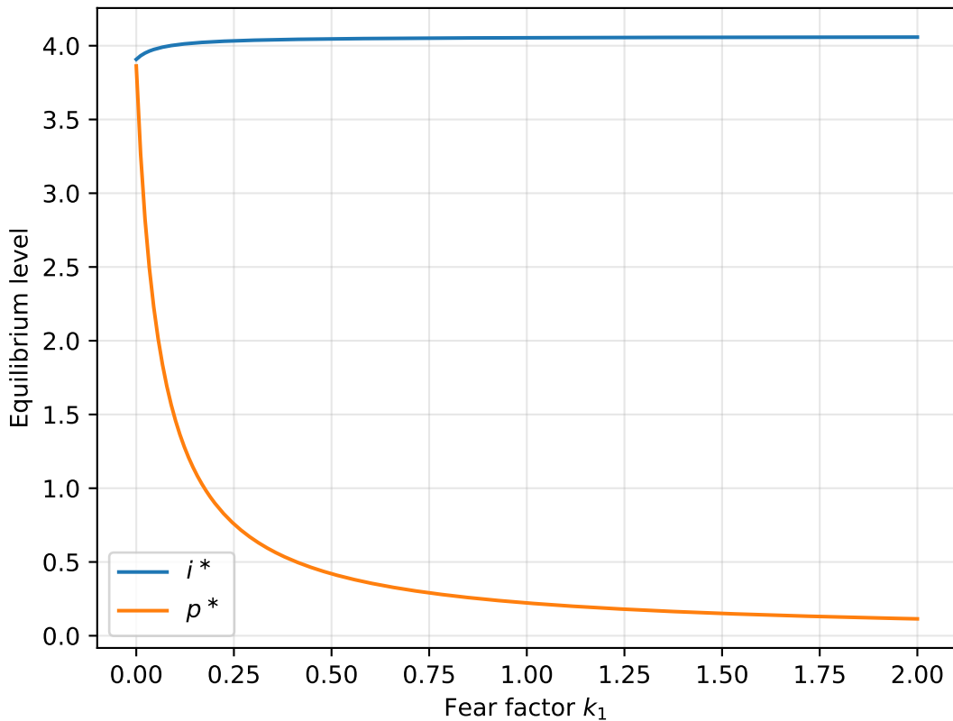
Effect of fear on coexistence equilibrium: i^* and p^* vs k_1
