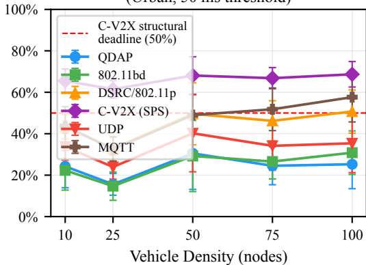
Emergency Message Deadline Miss Rate (Urban, 50 ms threshold)
