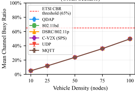
Channel Busy Ratio vs. Vehicle Density (Urban Scenario)
