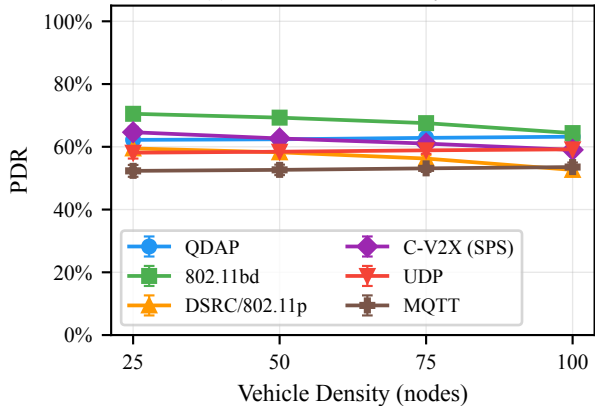
(a) BSM Packet Delivery Ratio
