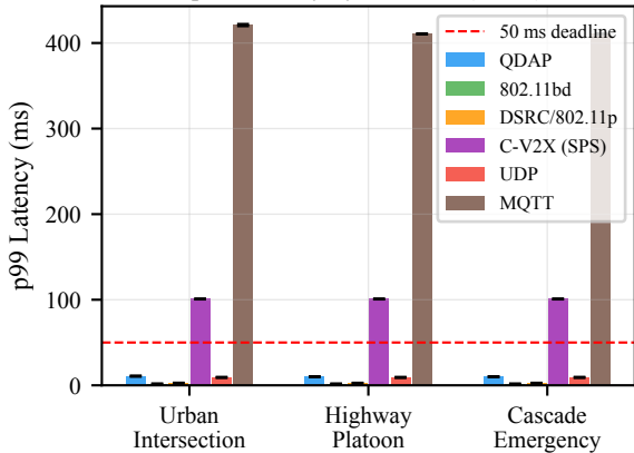
p99 Latency by Scenario (N=75)
