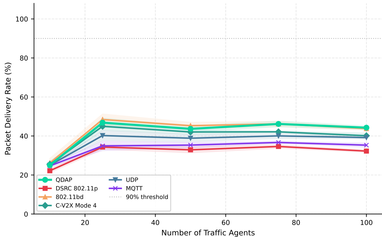
Emergency DENM Delivery Rate — Highway Platoon Scenario
