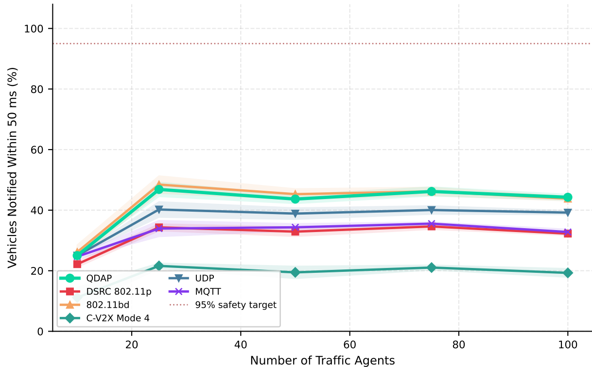
Safety: DENM Delivery Within 50 ms — Highway
