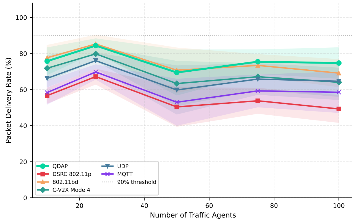
Emergency DENM Delivery Rate — Urban Intersection Scenario
