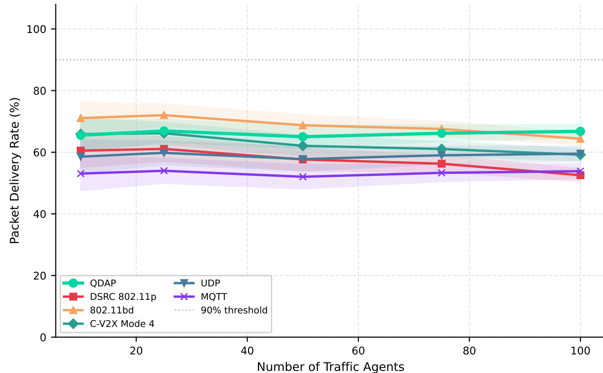
BSM Delivery Rate — Urban Intersection Scenario
