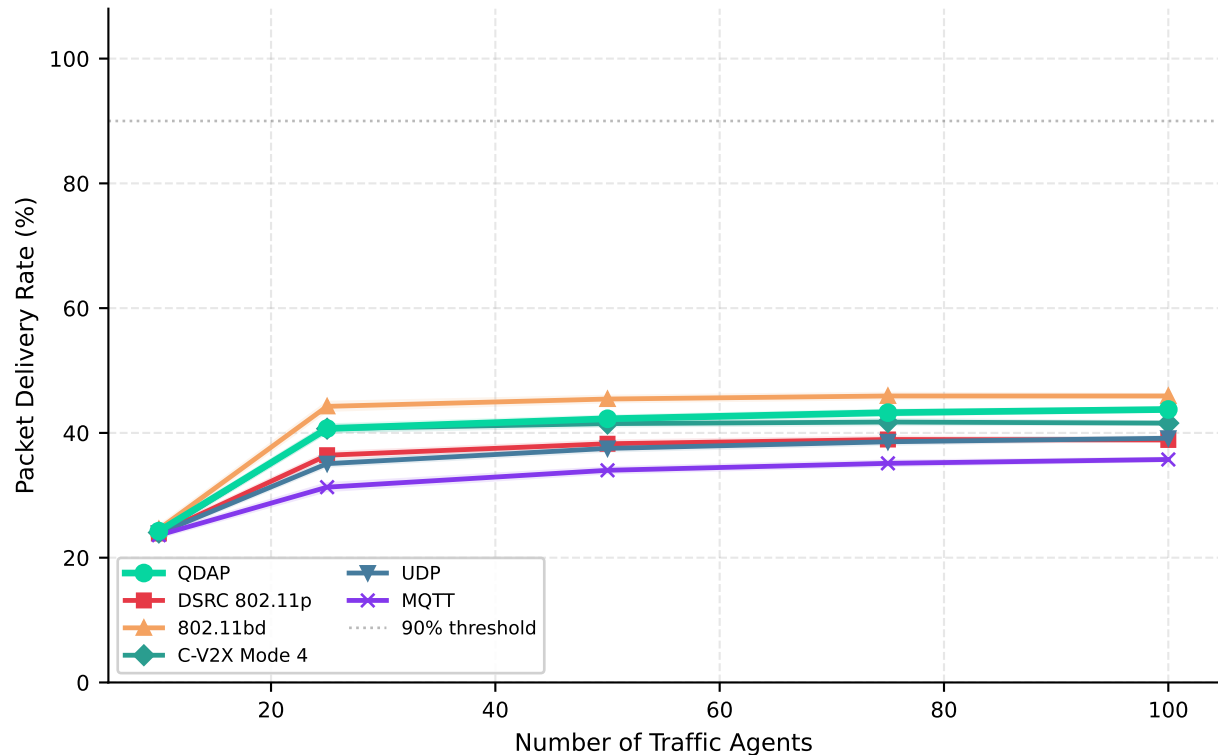
BSM Delivery Rate — Highway Platoon Scenario
