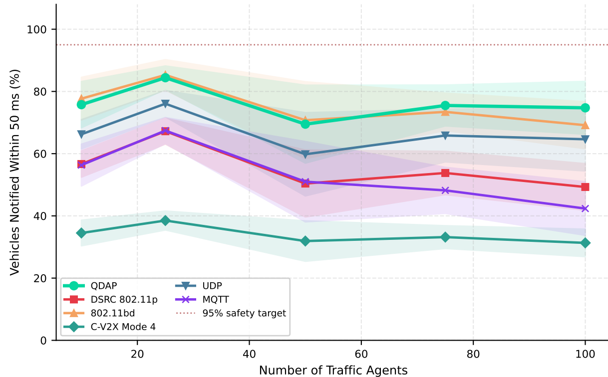
Safety: DENM Delivery Within 50 ms — Urban
