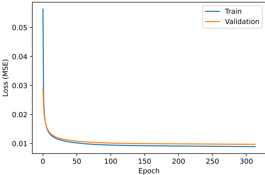
Learning Curve
