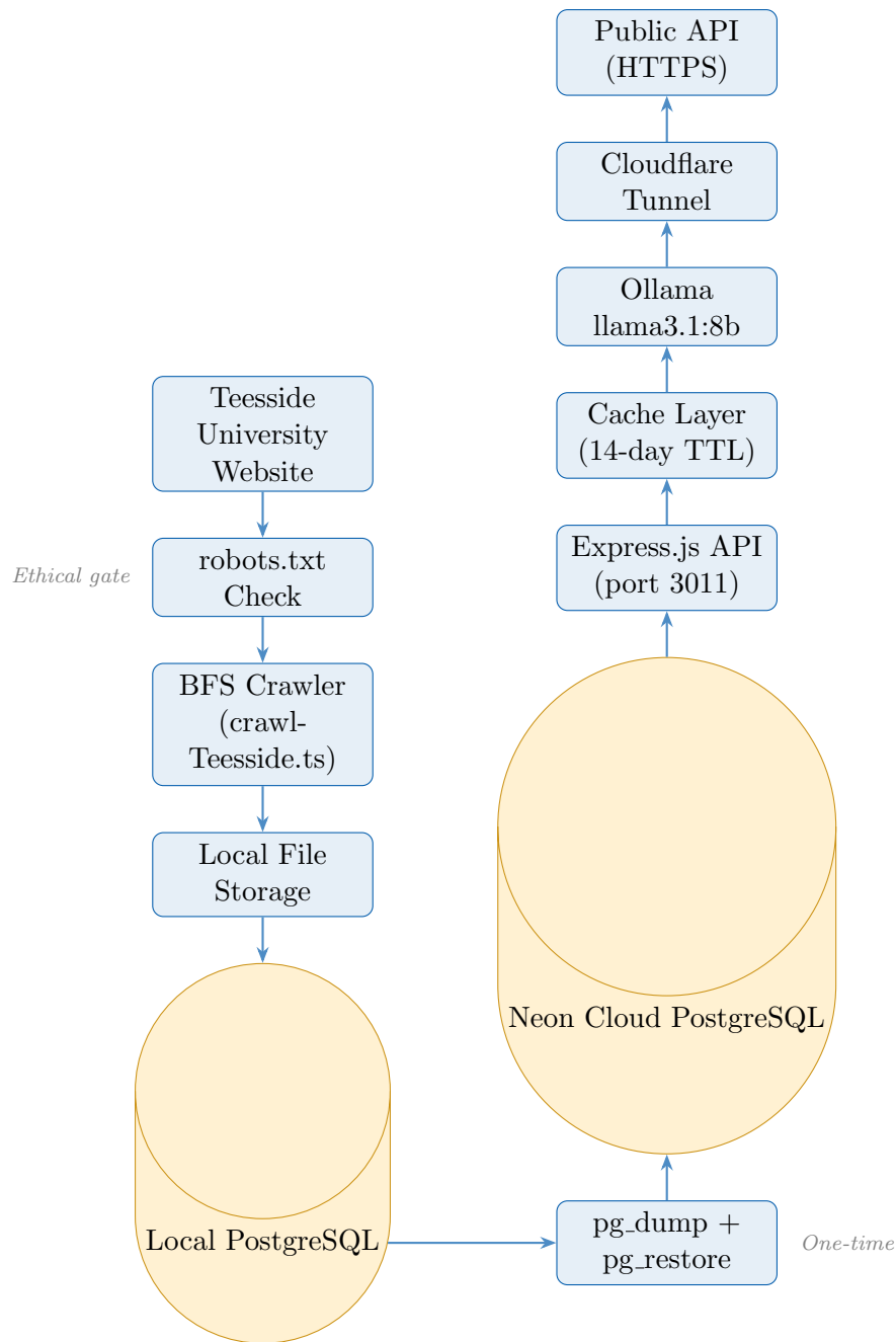
Figure 3.1: Complete CampusPaddy AI system pipeline from data collection to public API
