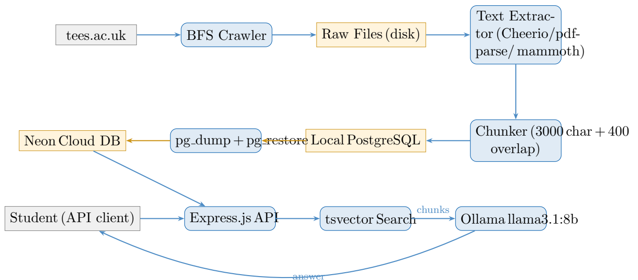
Figure 3.3: Data flow from university website to student answer
