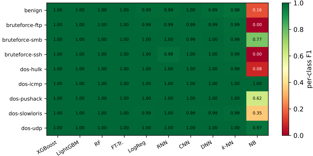
Per-class F1, audited condition (seed 1)
