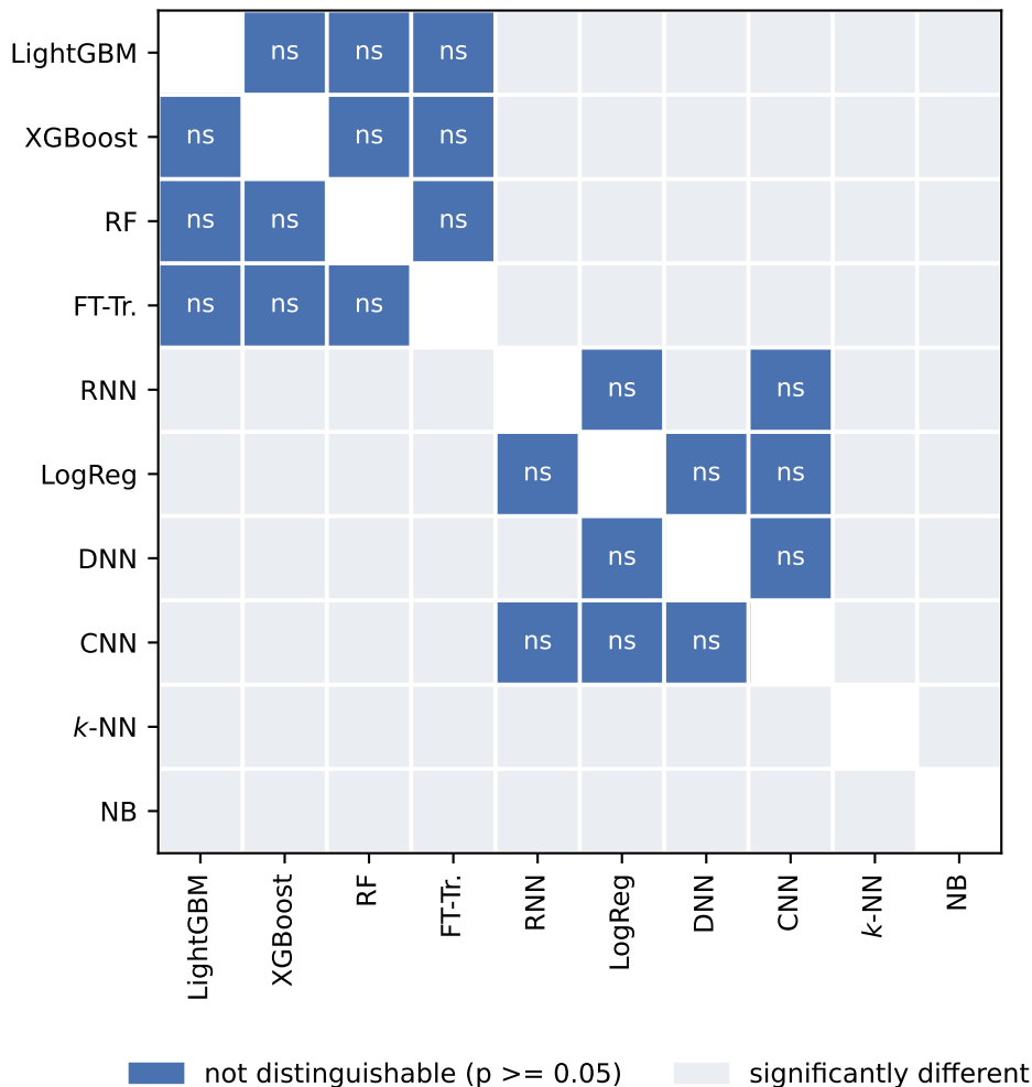
Saturation: 11 model pairs are not distinguishable (McNemar, Holm-corrected, \alpha = 0.05 ; models ordered by macro-F1)
