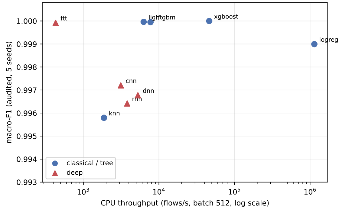
Inference cost versus detection quality
