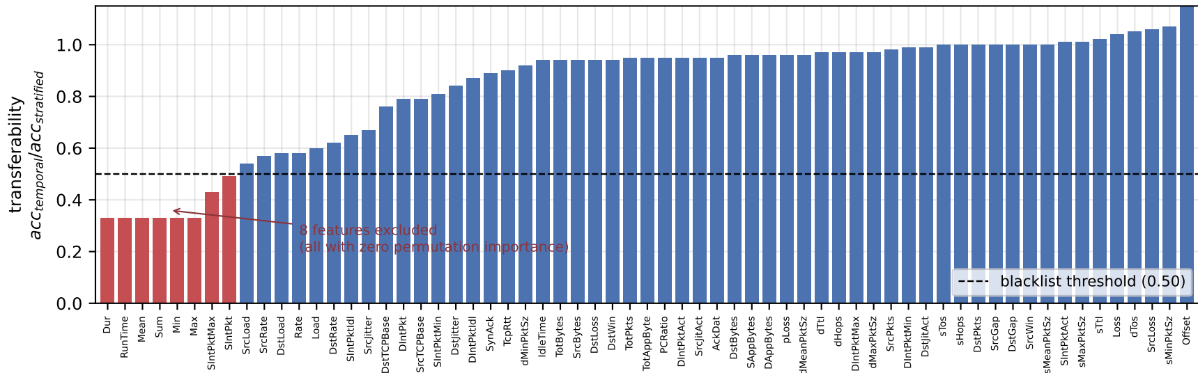
Single-feature transferability spectrum (63 behavioural features)
