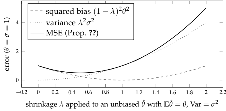
Figure 4.1: The bias–variance ledger: shrinking or capping an unbiased estimator ( \hat{\theta} \mapsto \lambda \hat{\theta} , or the truncations of Sections ?? and ??) buys variance at the price of bias; the MSE-optimal \lambda^* = \theta^2 / (\theta^2 + \sigma^2) balances the two curves, and truncation estimators sit at an interior point chosen so the bias lands inside the stated factor.
