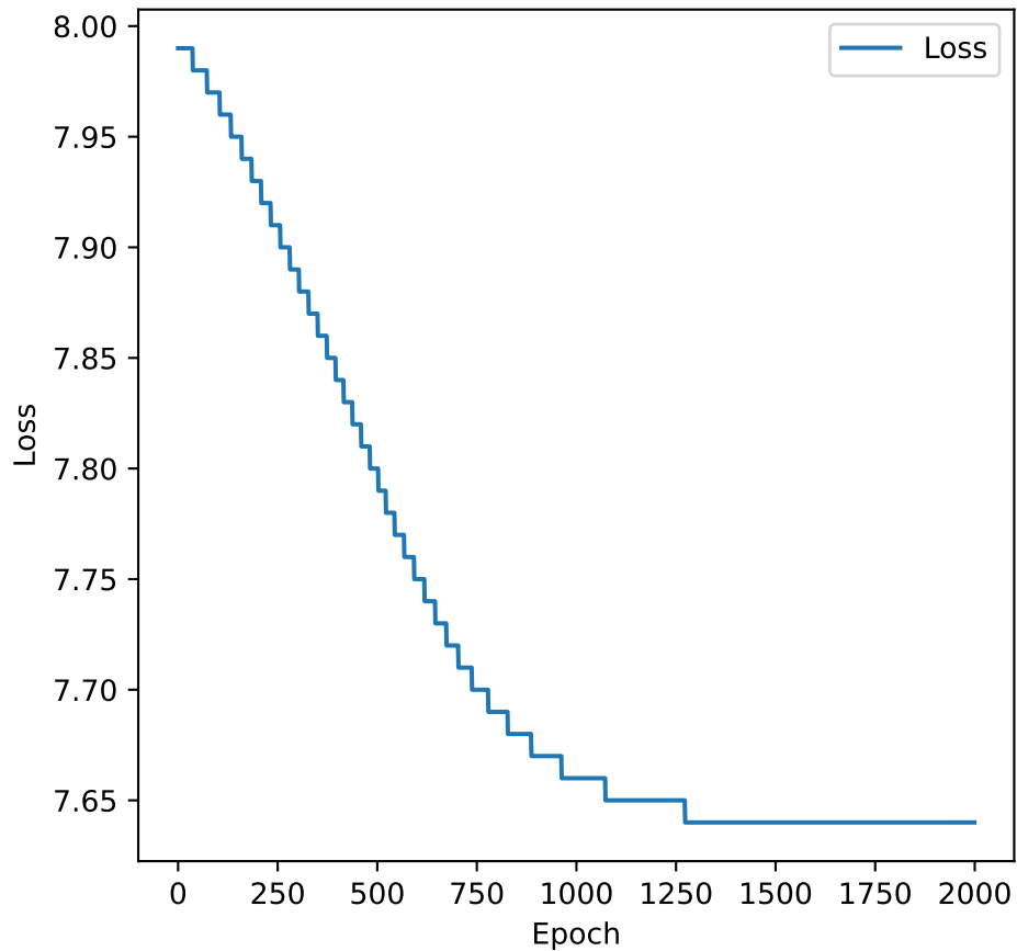
Training Loss
