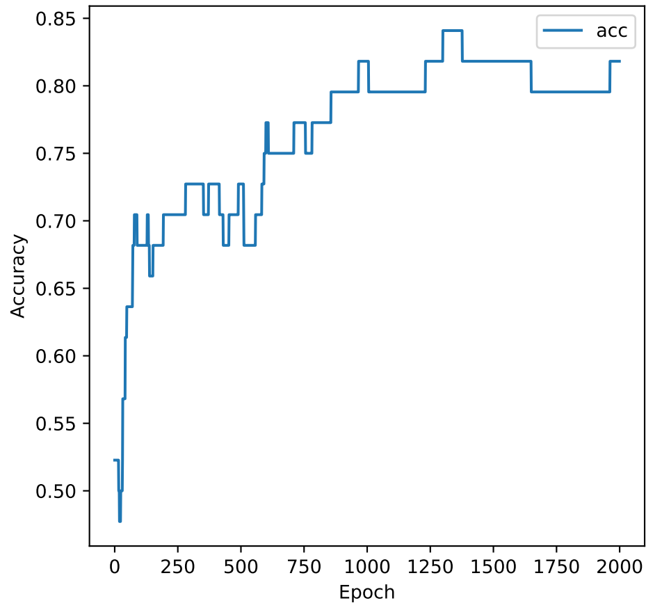
Training Accuracy
