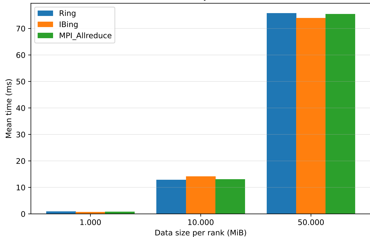
All-Reduce time by data size, N=3
