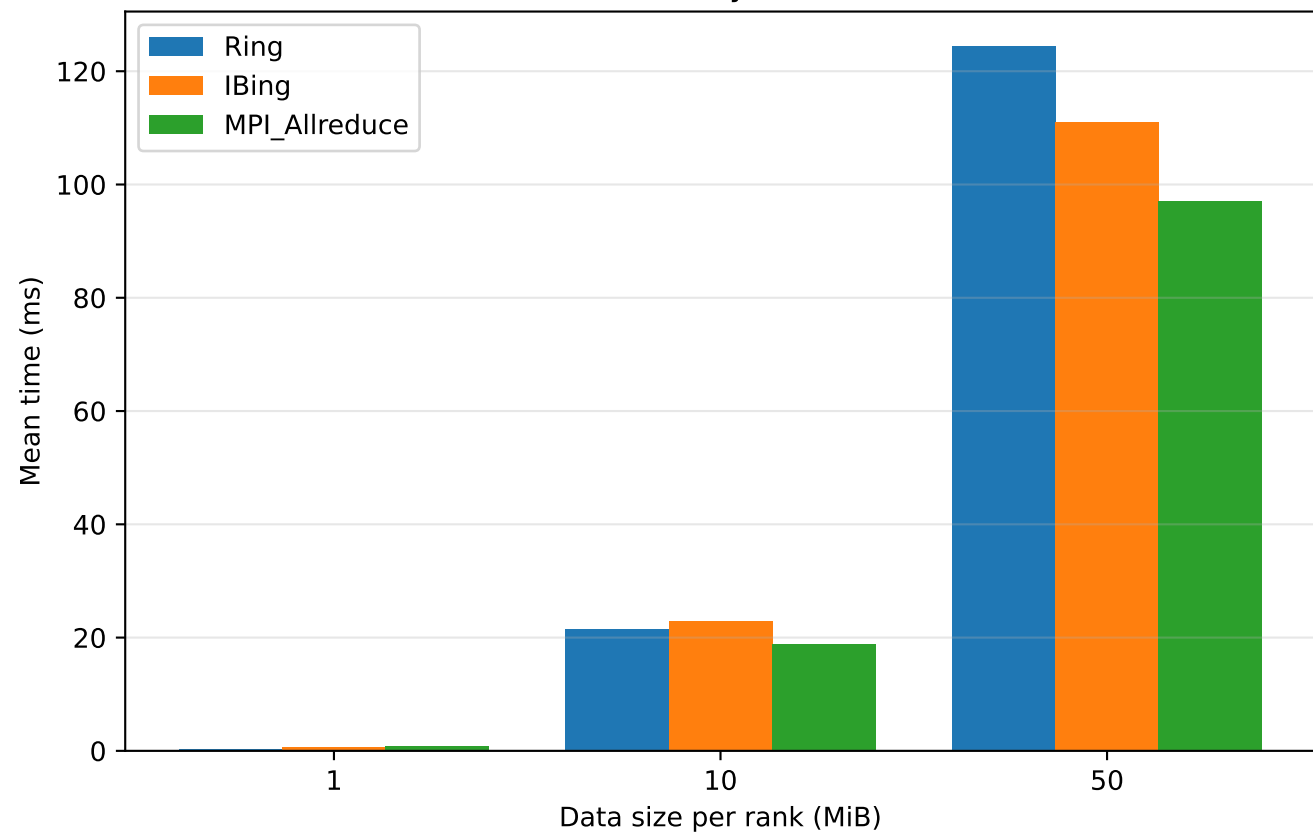
All-Reduce time by data size, N=4
