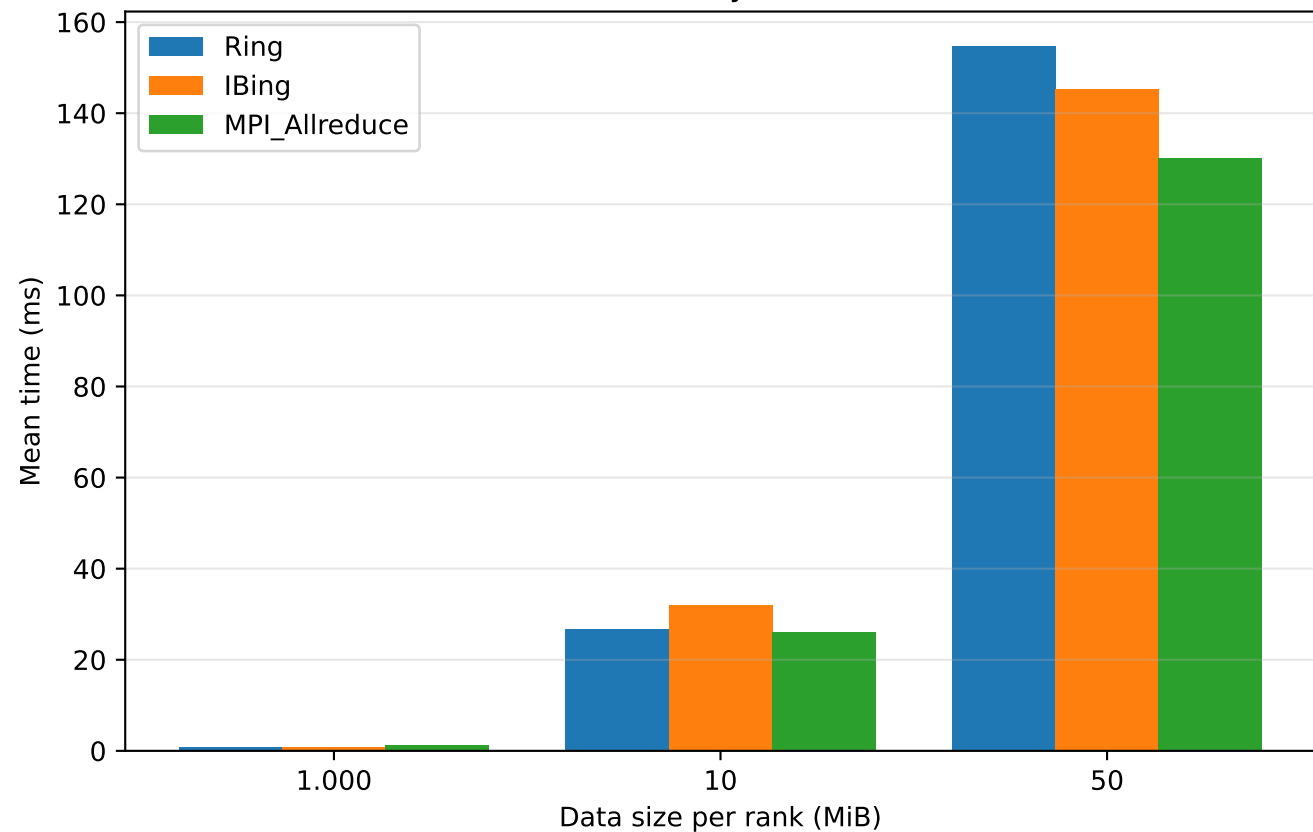
All-Reduce time by data size, N=5
