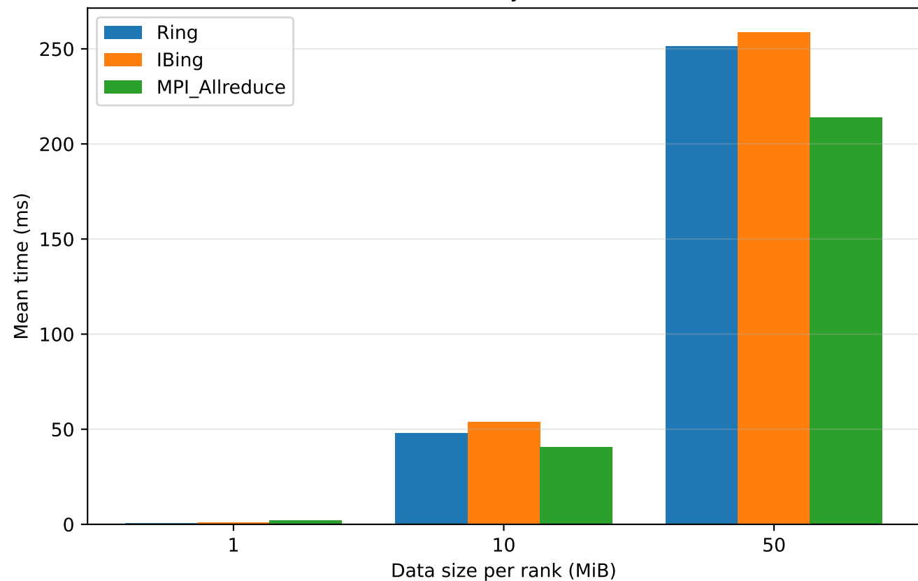
All-Reduce time by data size, N=8
