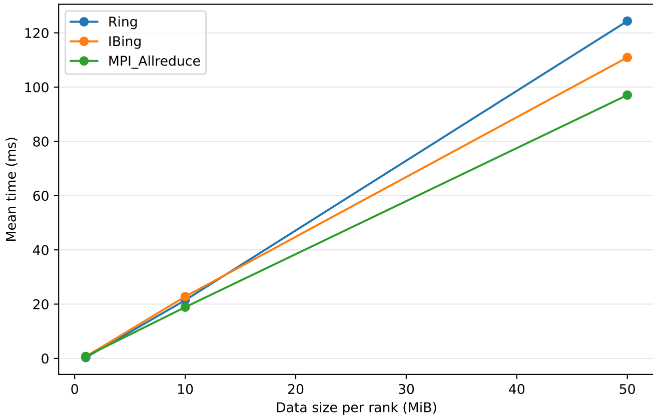
All-Reduce time comparison, N=4
