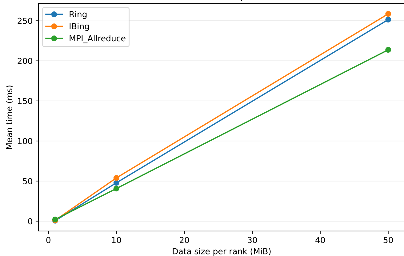
All-Reduce time comparison, N=8
