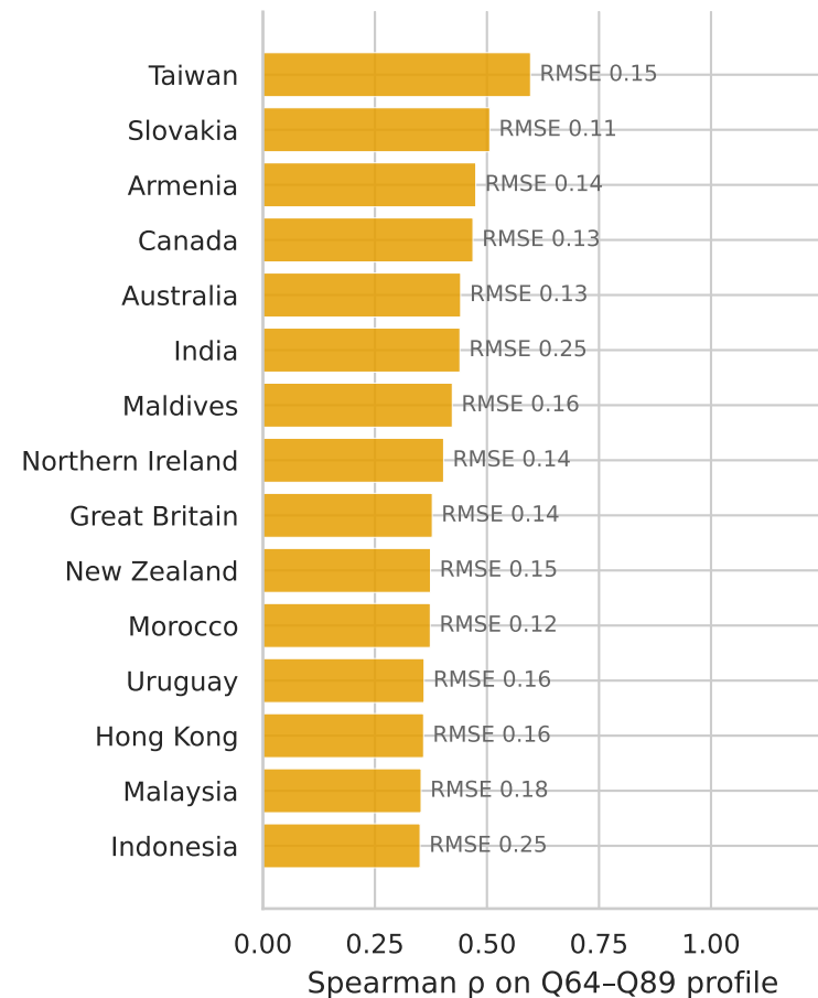
Figure 5 · Which WVS-7 country does each LLM resemble most on institutional trust?
