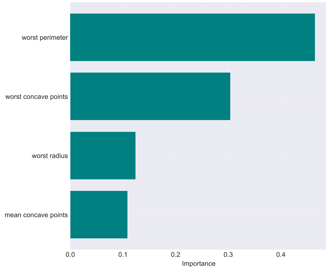
Top Features (AdaBoost)
