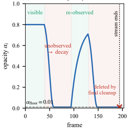
(b) reversible opacity, then deletion
