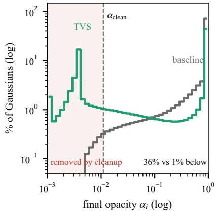
(a) opacity distribution
