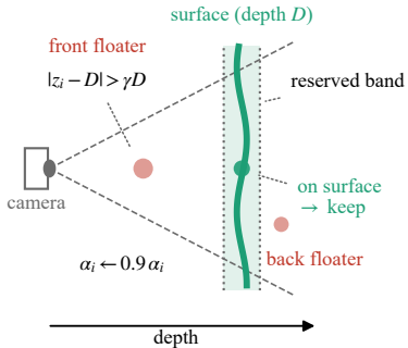
(c) spatial floater mask
