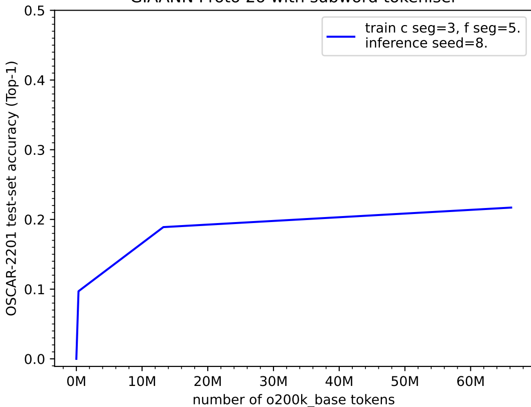
GIAANN Proto 2o with subword tokeniser
