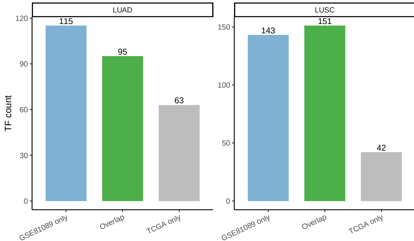
Supplementary Figure 2B – direction-concordant TF overlap
