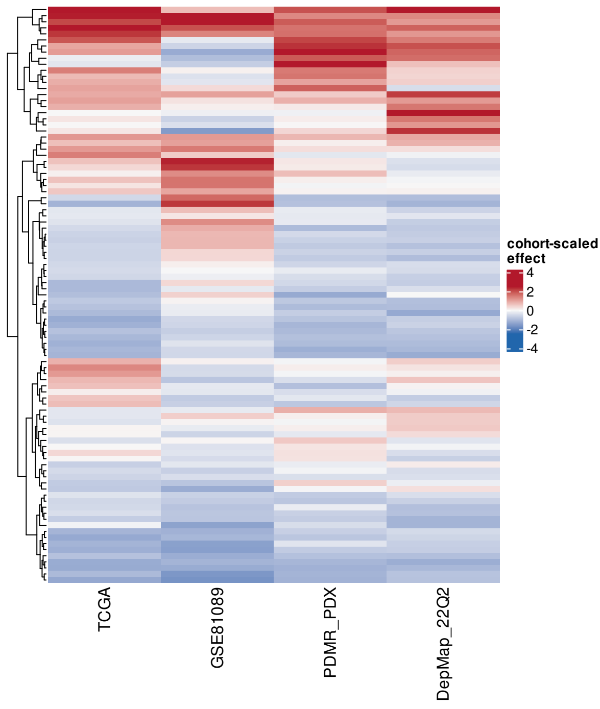
Supplementary Figure 2F — 95 externally replicated LUAD TFs
