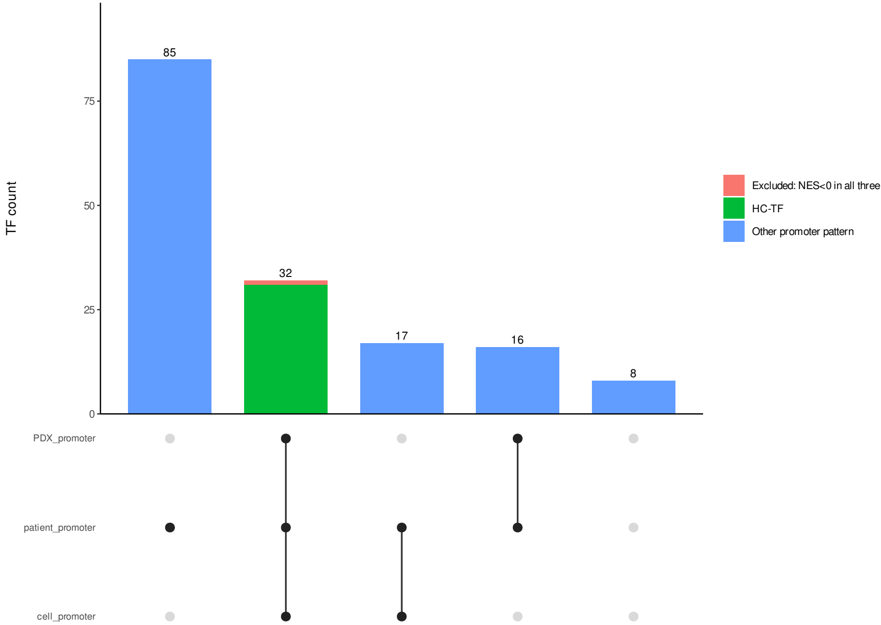
B Promoter combinations; all-three-negative NES exclusion highlighted
