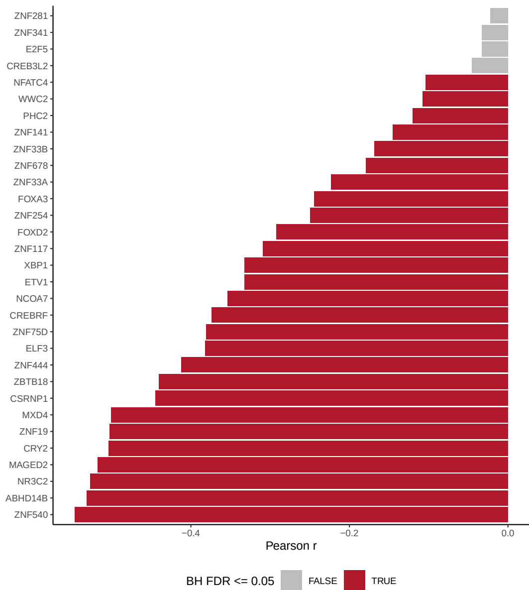
A HC-TF activity association with MKI67
