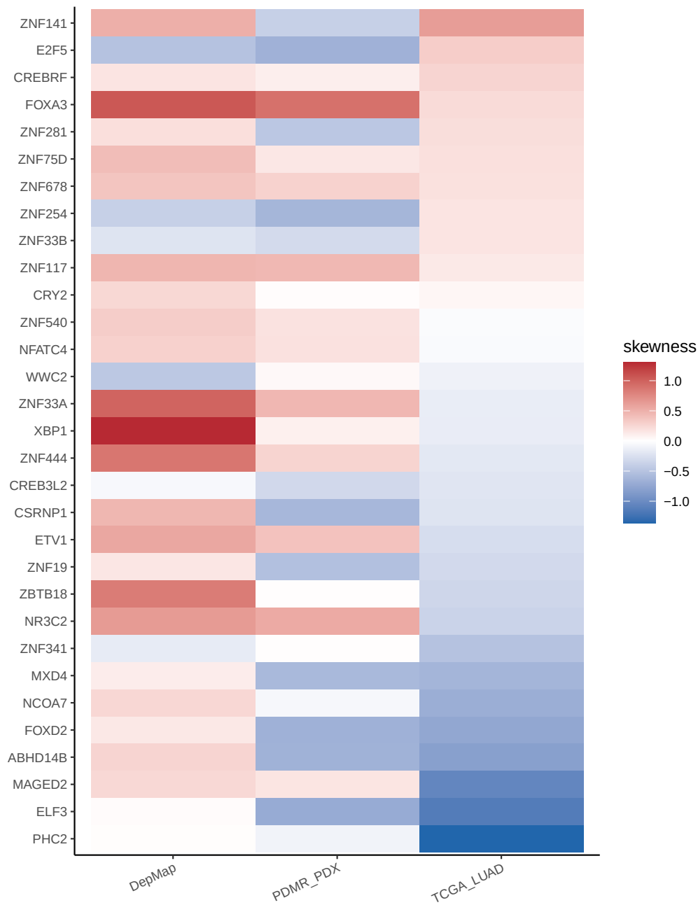
B HC-TF activity skewness across LUAD systems
