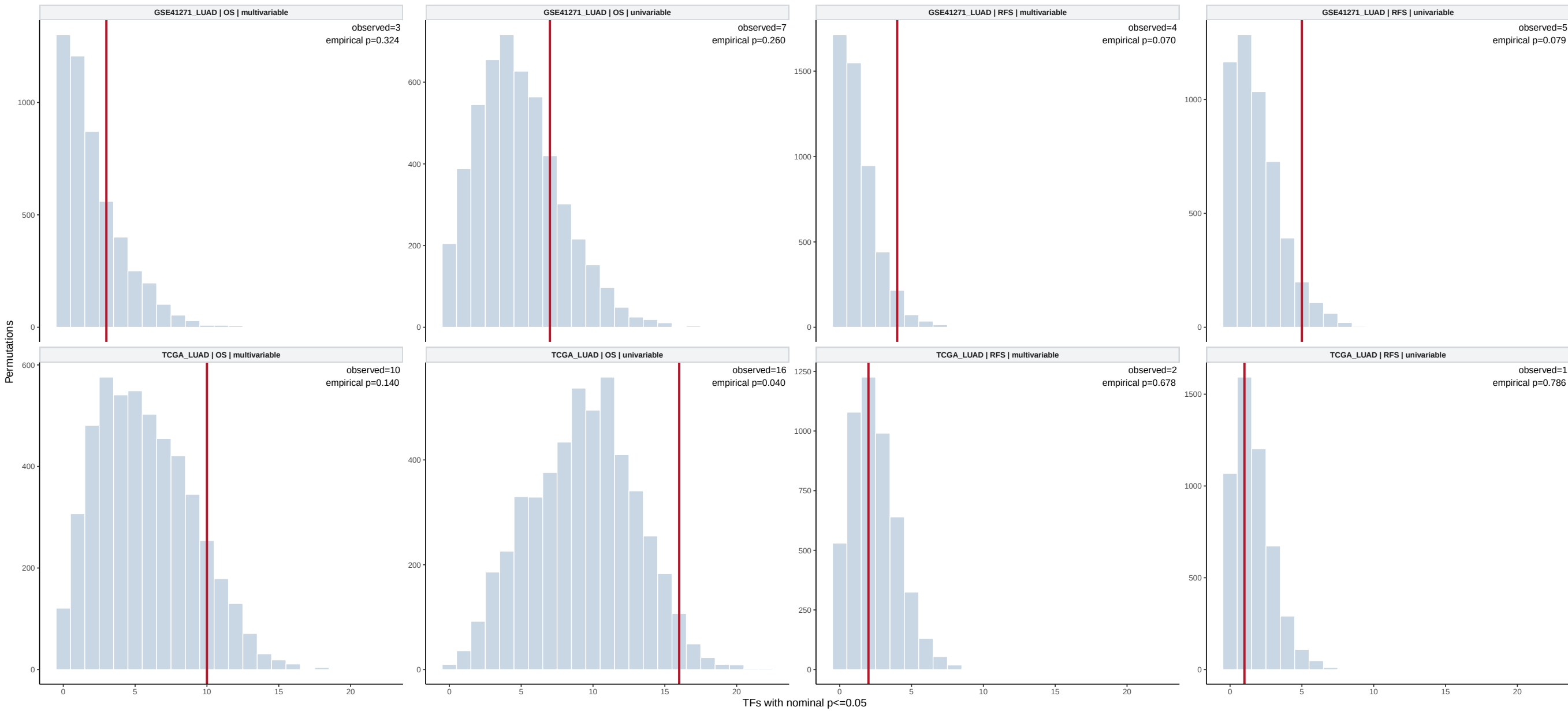
Supplementary Figure 6I-P | Five-thousand-permutation null distributions
