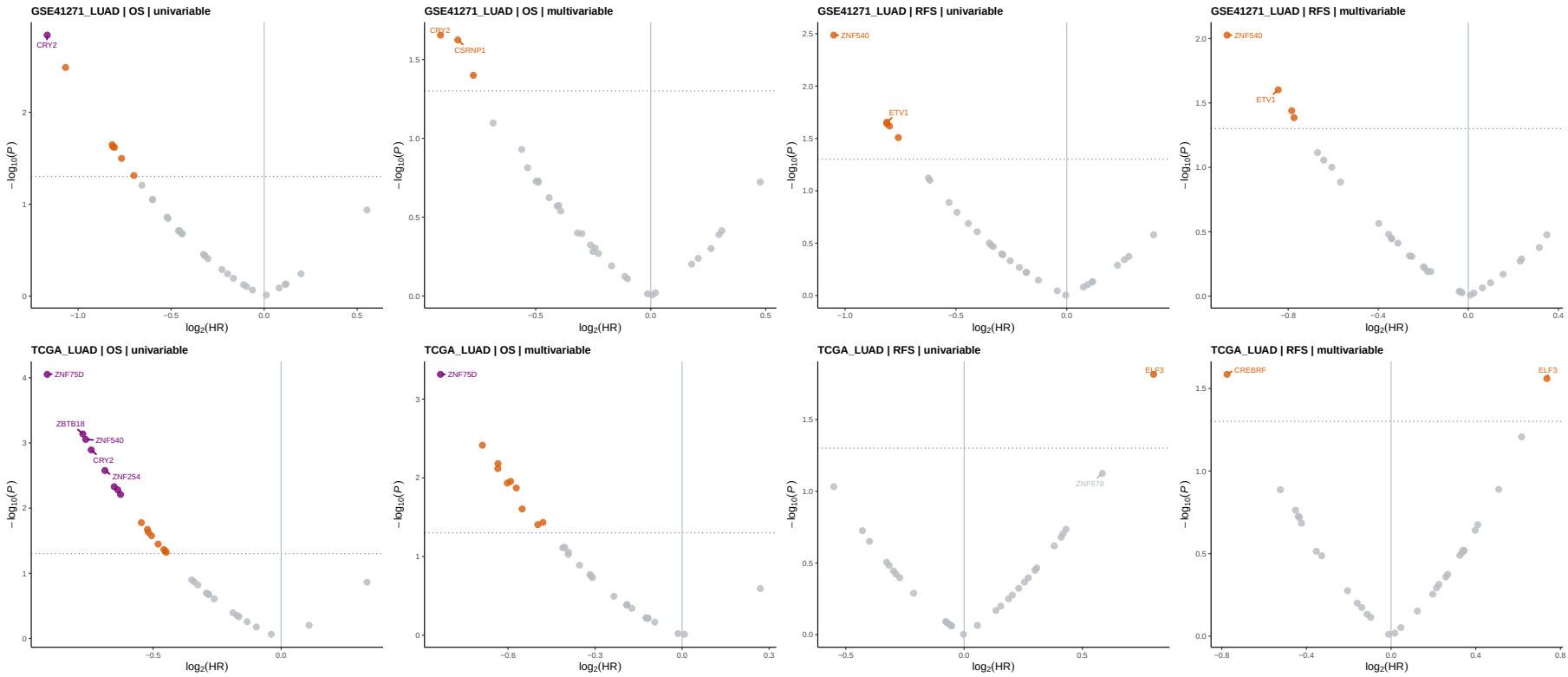
Supplementary Figure 6A-H | Continuous-activity Cox screens Purple: BH FDR<=0.05; orange: nominal p<=0.05; all 31 HC-TFs are displayed
