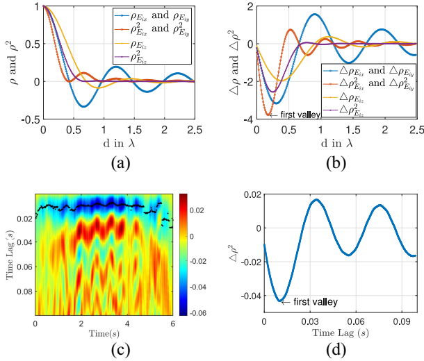
Fig. 2. Spatial ACF and its differential for EM wave components. (a) Theoretical spatial ACFs. (b) Theoretical differential of spatial ACFs. (c) Differential ACF of response power and the valley location. (d) Instance of differential spatial ACF of response power.
