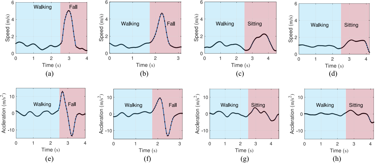
Fig. 7. Instances of speed and acceleration patterns for “walk-then-fall” and “walk-then-sit” (a) and (e) Speed and acceleration for “walk-then-fall” under LOS. (b) and (f) Speed and acceleration for “walk-then-fall” under NLOS. (c) and (g) Speed and acceleration for “walk-then-sit” under LOS. (d) and (h) Speed and acceleration for “walk-then-sit” under NLOS.
