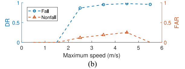
Fig. 15. Maximum speed distribution and DR/FAR for each maximum speed interval. (a) Distribution based on the maximum speed. (b) DR/FAR in each maximum speed interval.
