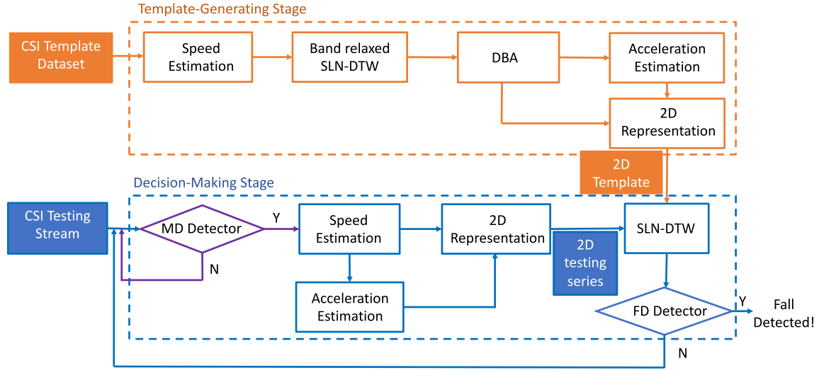
Fig. 3. Overview of DeFall.
