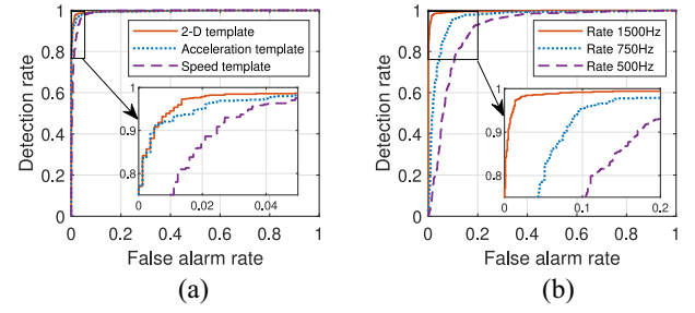
Fig. 14. ROC curves for (a) comparison on 2-D template and 1-D separate templates and (b) different sampling rates.
