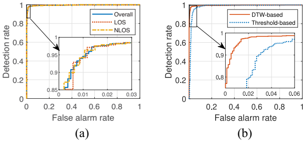
Fig. 10. ROC curves for (a) different scenarios and (b) comparison with the threshold-based method in WiSpeed.
