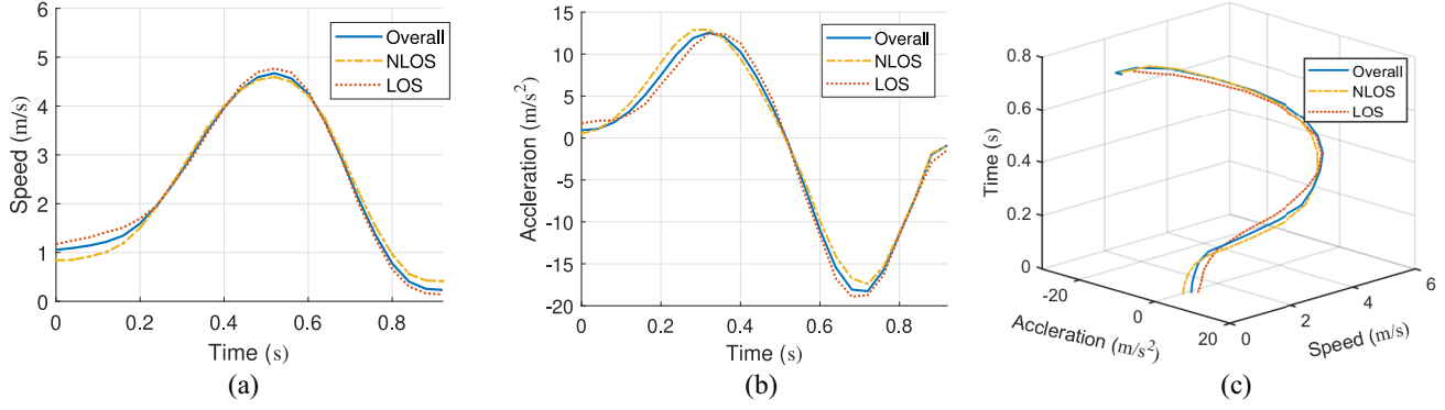
Fig. 9. Templates. (a) Speed templates. (b) Acceleration templates. (c) 2-D templates.
