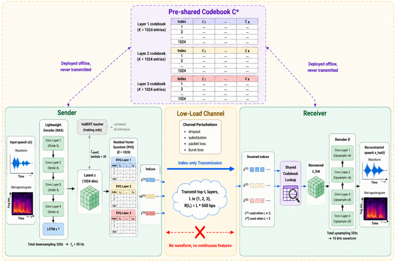
Fig. 1. SCIT-Speech system overview. The transmitter and receiver pre-share the RVQ codebooks C^* , decoder D , and configuration. Runtime packets contain only the first L layers of RVQ indices. LCA trains the shared decoder to reconstruct robustly from truncated and perturbed index sequences; the HuBERT teacher is used only during Base training.
