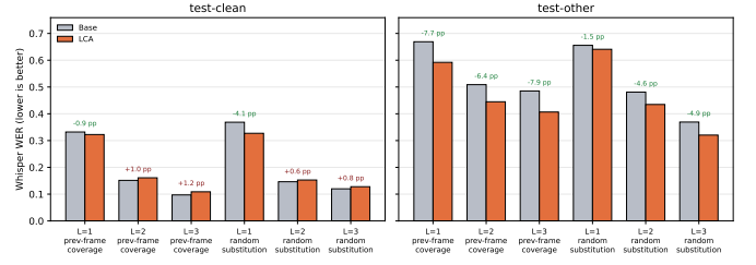
Fig. 5. Whisper WER under high index perturbations. The annotations show LCA minus Base in percentage points. LCA consistently improves test-other, while test-clean gains are concentrated at L = 1 .
