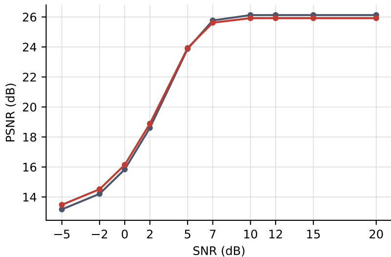
(c) k = 4 PSNR under AWGN
