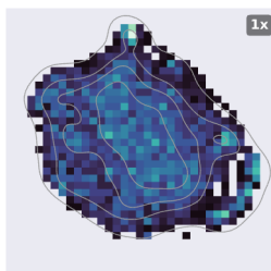
BBDRec
