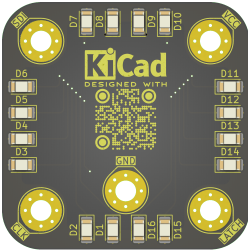
PCB: Sienkiewicz LED
