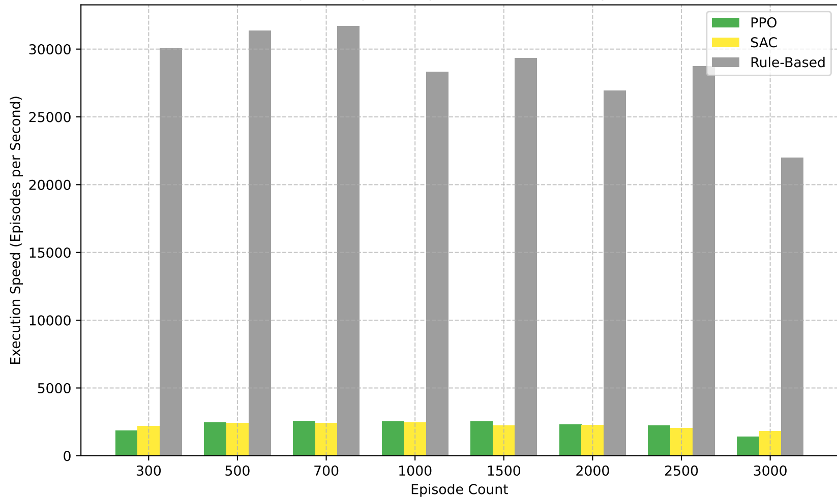
Execution Speed (Episodes per Second) Across Episode Counts
