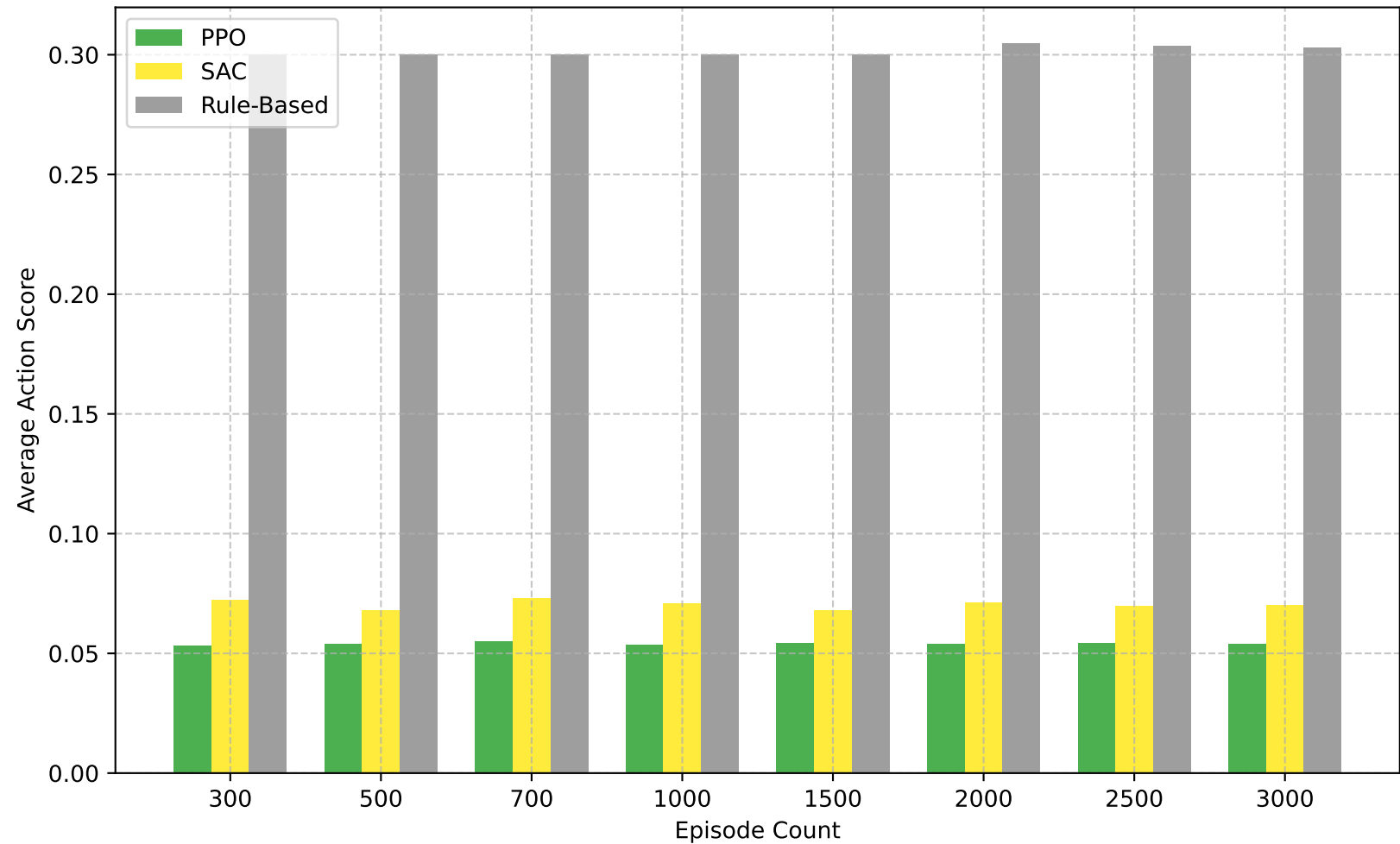
Average Action Score Across Episode Counts
