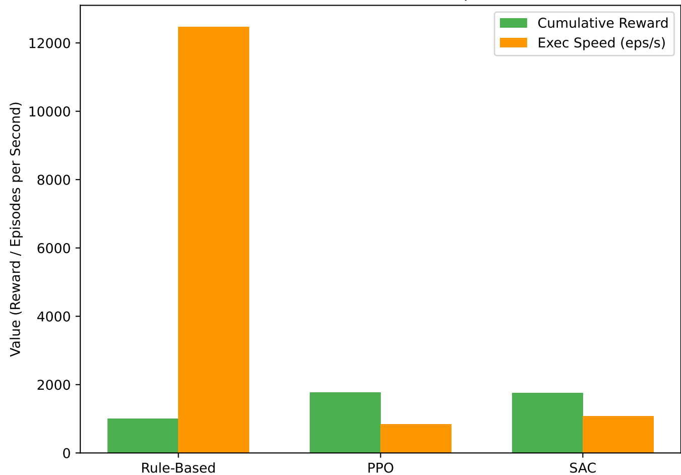
Performance Metrics (2000 Episodes)
