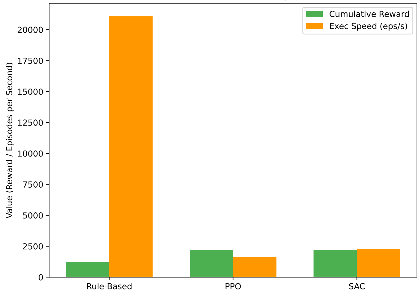
Performance Metrics (2500 Episodes)
