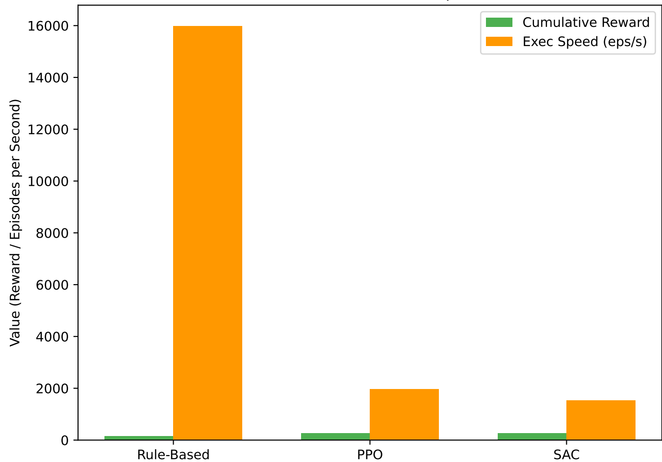
Performance Metrics (300 Episodes)
