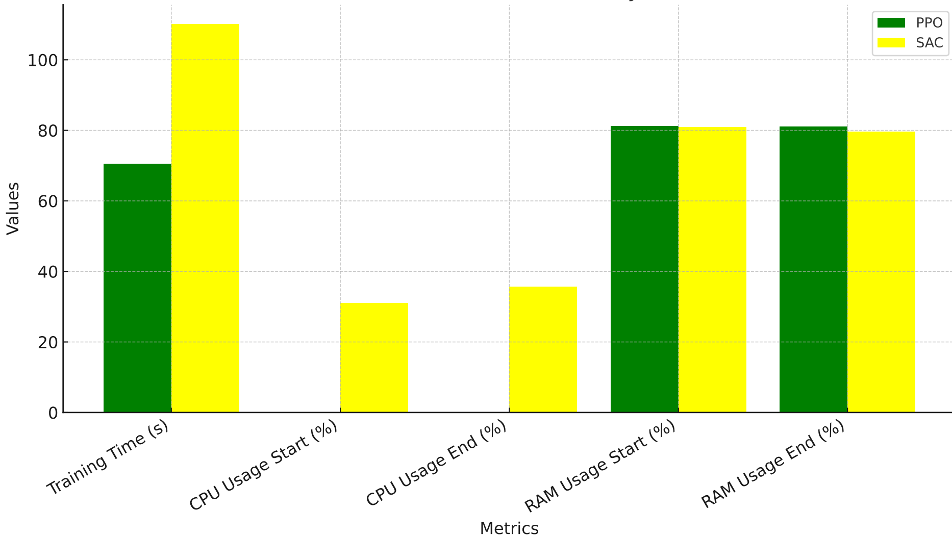
PPO vs SAC Runtime Analysis
