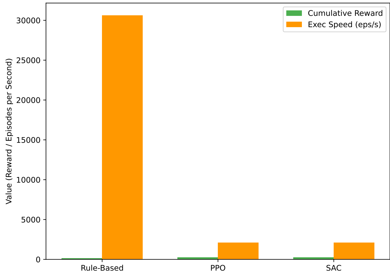
Baseline vs. PPO vs. SAC: Performance Metrics
