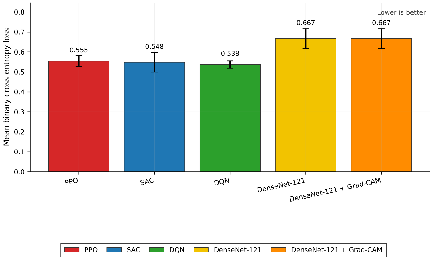
Final predictive loss: adaptive agents versus baselines
