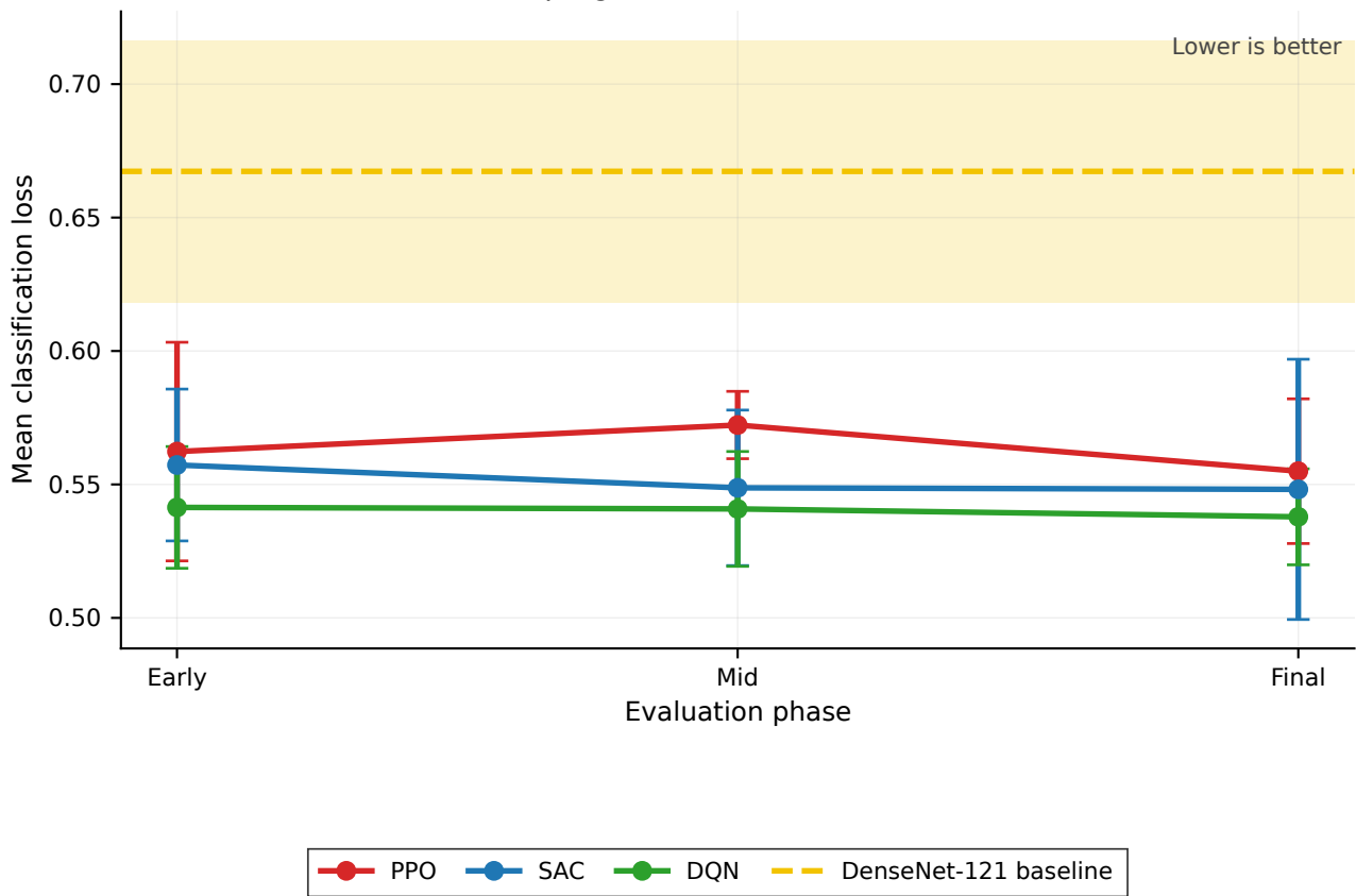
Predictive loss progression with DenseNet-121 reference
