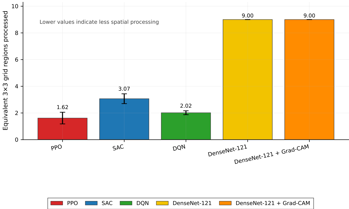
Adaptive regional inspection versus full-image processing
