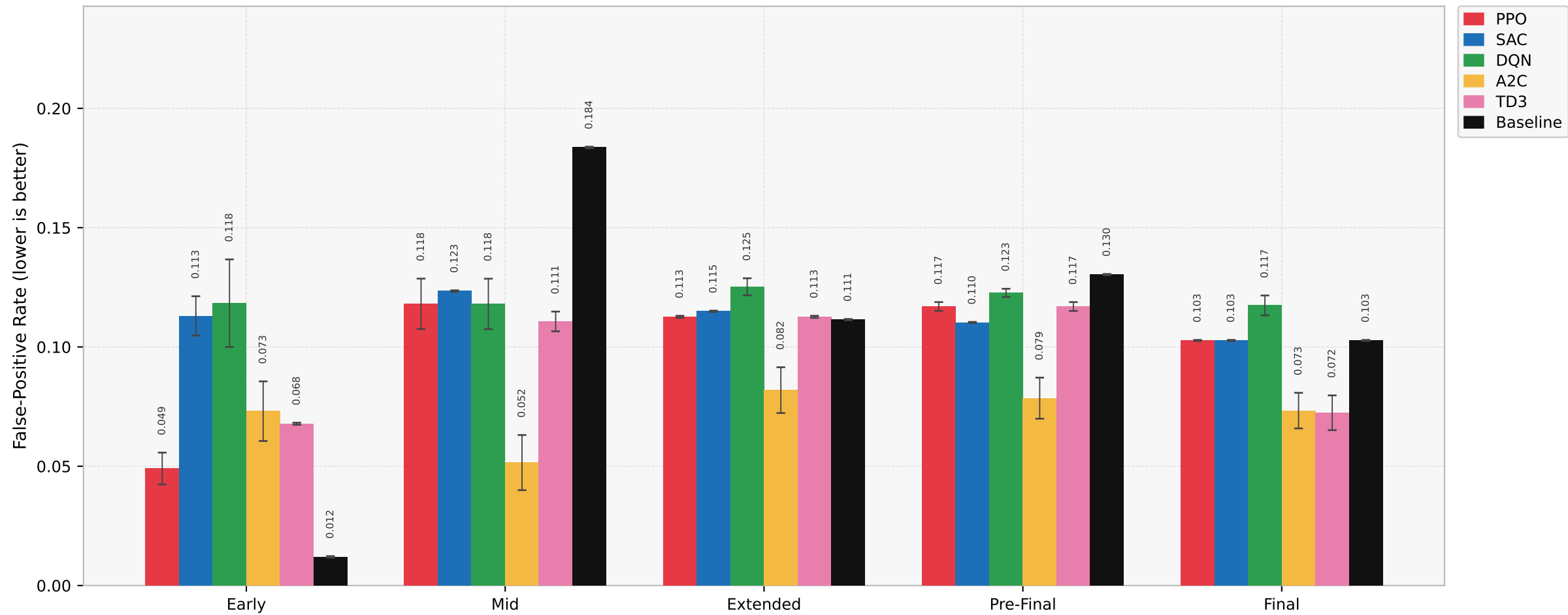
False-Positive Rate per Phase and Algorithm (mean +/- 95% CI, 3 seeds)
